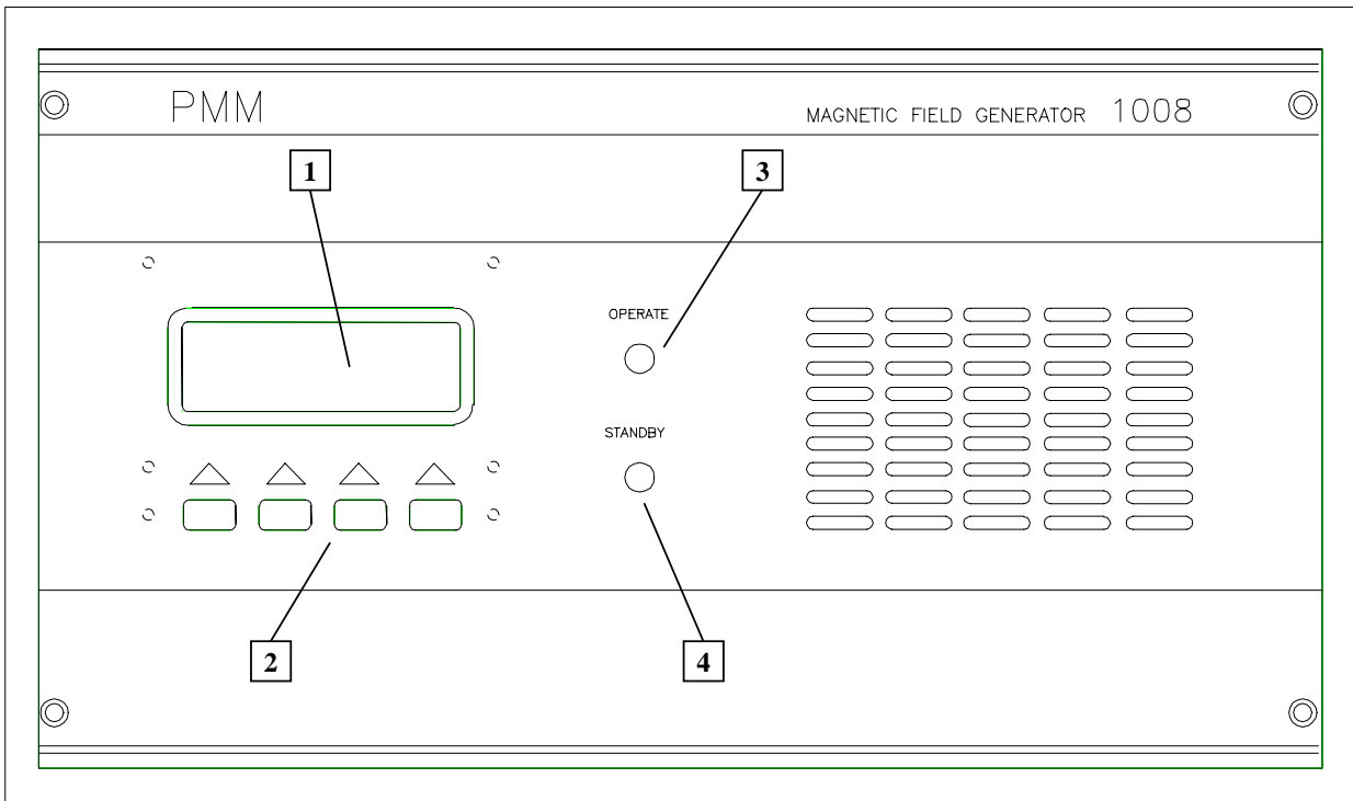
Fig. 1-2 Front Panel
