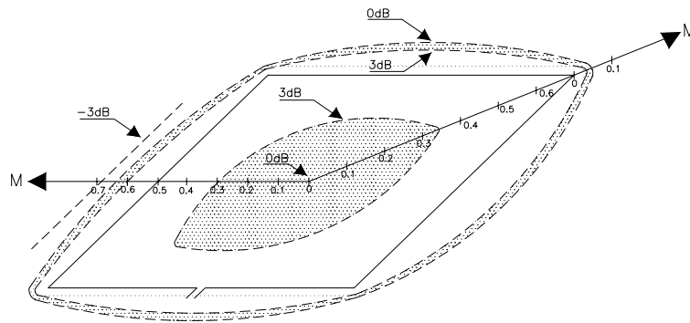
Fig. 4-2: 3dB area of the field generated by a square induction coil (1m side) in its plane
